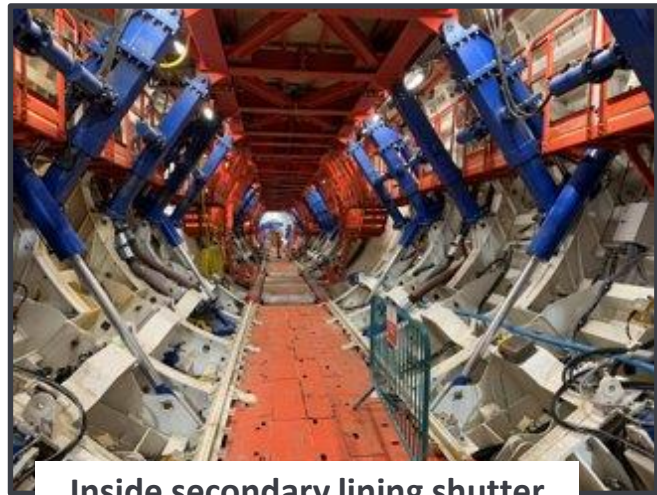
Inside secondary lining shutter
