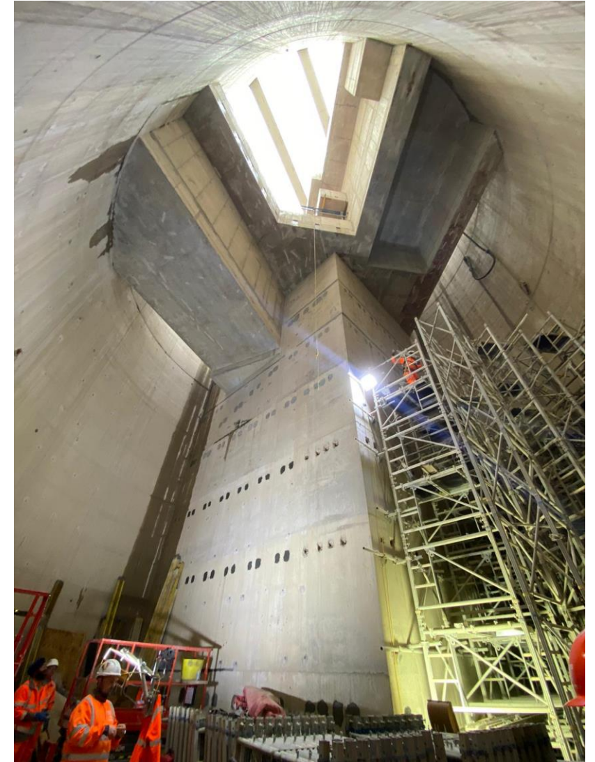
CSO Shaft Internals (Inc Vortex Tubes, SWSR Portal and Culvert Portal)
